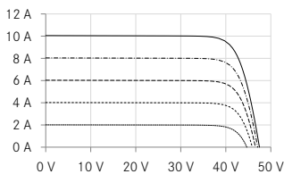
UP-diagramm e.g. LX-370M/156-72+
