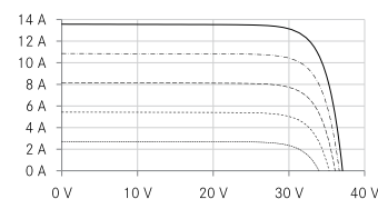
UI-diagram e.g. LX-410M/182-108+
