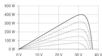
UI-diagram e.g. LX-410M/182-108+
